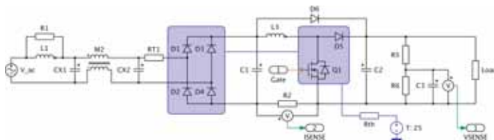
Figure 2. Schematic of a switch mode power supply
