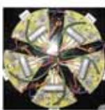
3-phase drive unit
